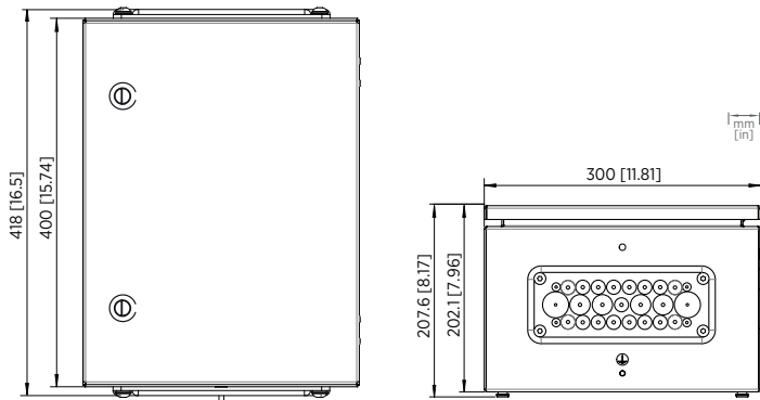
Figure 6 CAB100A enclosure dimensions
