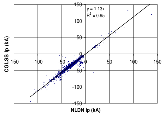
Figure 5. CGLSS I_p values vs. the corresponding NLDN I_p values.
