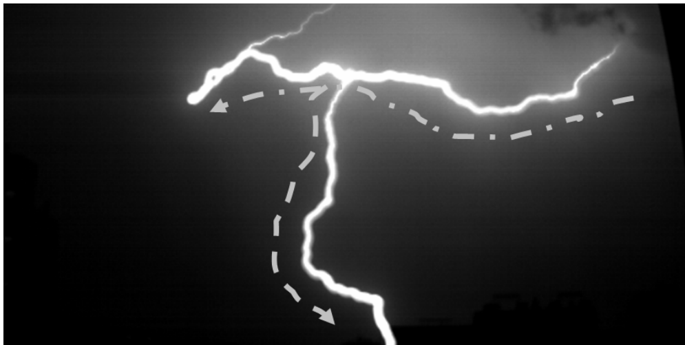
Figure 1. Image of a positive leader emanating from a previous horizontal channel (Tucson, 03:24 UT, July 31, 2007, 6 km from the camera). The dashed arrows show the directions of progression of the horizontal and vertical leaders.
