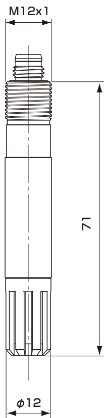
HMP110/HMP110T
